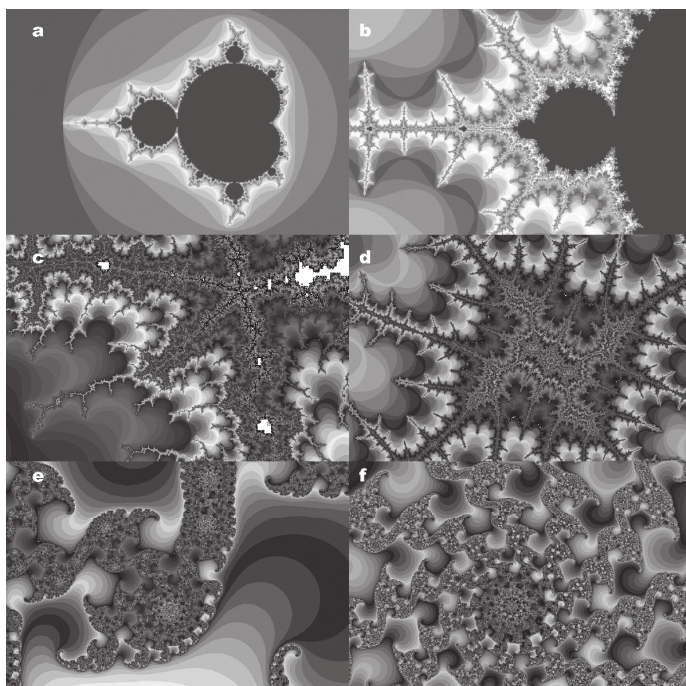
Fig. 5.1 Graphical depiction of the Mandelbrot set (a). This set includes elements that belong to the plane of complex numbers (in the figure, the abscissa corresponds to the real part and the ordinate corresponds to the imaginary part of a particular complex number c ) that, even after infinitely repeated substitution into the (recurrent) equation z_{n+1} = z_n^2 + c (where z_0=0 ), does not exceed a value of 2. Some points in the plane exceed a value of 2 in the very first substitution into the equation, while this occurs for others only when the given procedure, meaning addition to its square and substitution of the result into the right-hand side of the equation, is repeated many times. The number of these iterations necessary to exclude that a particular point belongs in the Mandelbrot set is shown in the figure by the darkness of gray. (A much nicer picture is formed when the number of iterations is depicted by various colors.) The areas in the plane of complex numbers for which 170 iteration steps still did not lead to exceeding a value of 2 and that could thus belong in the Mandelbrot set are depicted in black in the figure. This simple algorithm leads to an extremely complicated shape whose individual parts can be constantly zoomed in and further and further details can be found in them (b, c, d). The figures were created using the excellent program XAOS, which was available for free in 2017 on the web site http://matek.hu/xaos/doku.php .
