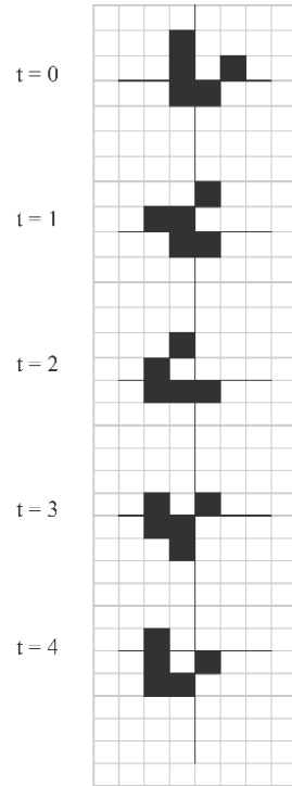
Fig. 5.3 Stable shapes are formed in the mathematical Game of Life. Among the patterns formed in the Game of Life, various types of “gliders”, the stable structures that move across the playing board, are quite remarkable. A “spaceship” remains stable until it collides with some other shape and until it reaches the edge of the playing board, meaning it is cyclically converted into several shapes. The figure shows a simple glider that, in four steps, always moves one square diagonally downwards to the left.
